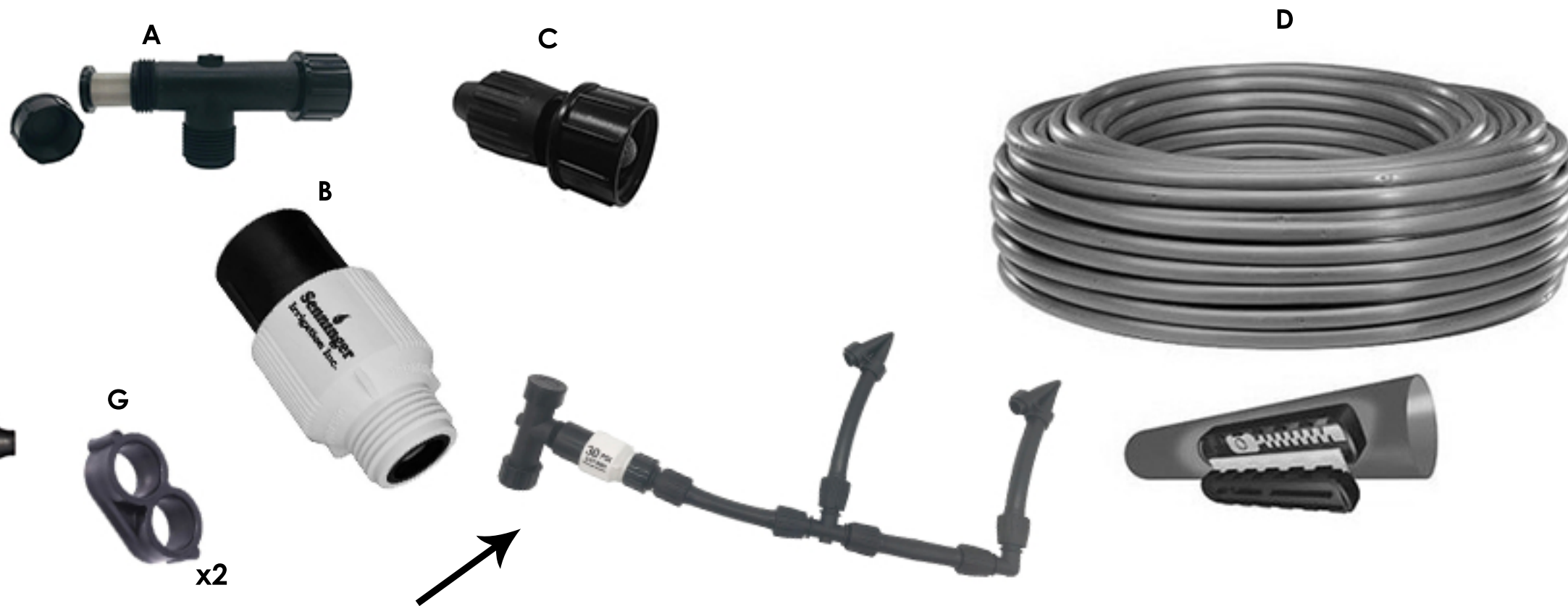
* Typical Hook-Up/Layout (Filter A, Regulator B, and Hose Swivel C shown connected to the In-Line Drip Hose)
