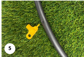
5 Use hole punch (F) to punch a hole in the side wall of the poly supply hose (D).
